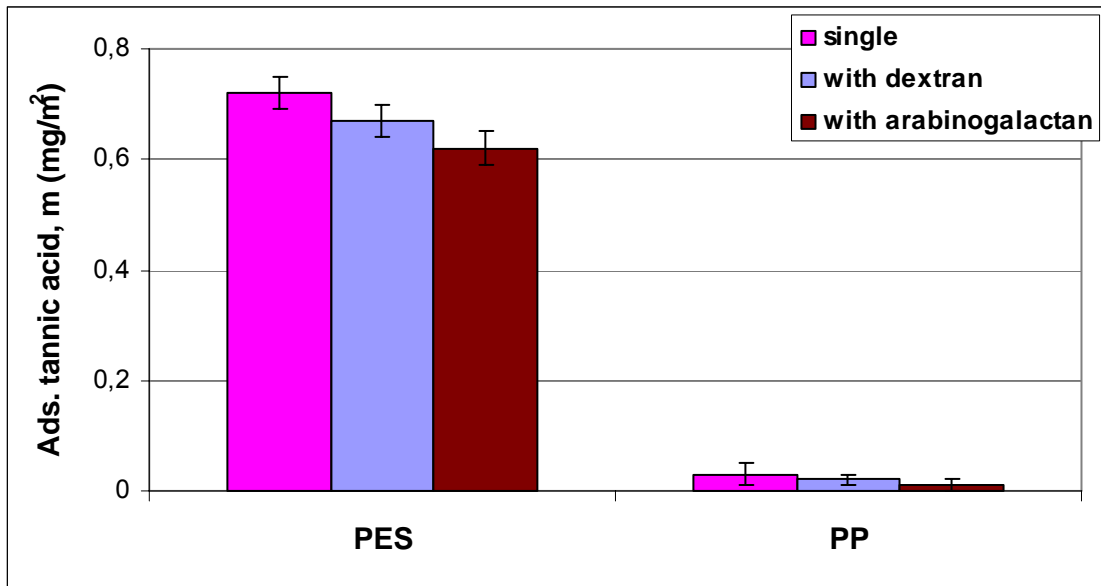
Figure 4: Adsorption of tannic acid (0.1 g/L) from single solute solution and mixtures with arabinogalactan or dextran (1 g/L; in “synthetic wine”) to PES and PP membranes (#1 and #2), relative to the membrane specific surface area.
