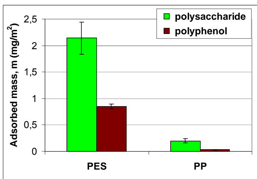
Figure 6: Adsorption of polysaccharide and of polyphenol from “synthetic red wine” (4 g/L) to PES and PP membranes (#1 and #2), relative to the membrane specific surface area.
