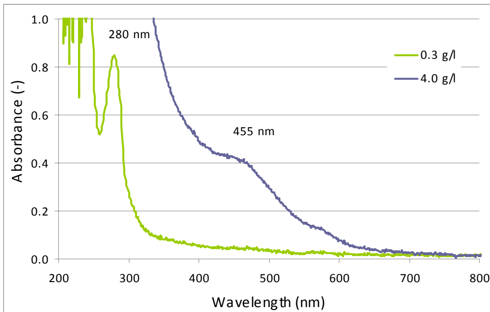
Figure 2: UV-Vis spectrum of „synthetic red wine“ (two different concentrations, cuvette thickness 1 cm).
