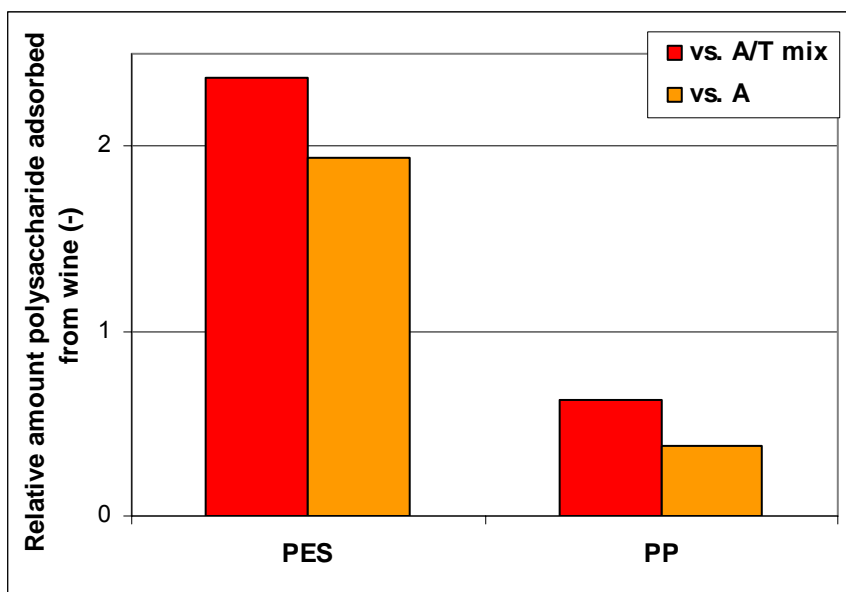
Figure 7: Relative amount of adsorbed polysaccharide from “synthetic red wine” (4 g/L) to PES and PP membranes (#1 and #2), in comparison to experiments with model solutions: “A/T mix” ... mixture of arabinogalactan (1 g/L) and tannic acid (0.1 g/L) in “synthetic wine”; “A” ... arabinogalactan (1 g/L) in “synthetic wine”.
